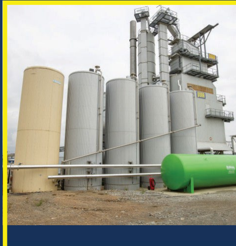
Sibiu Asphalt Plant
